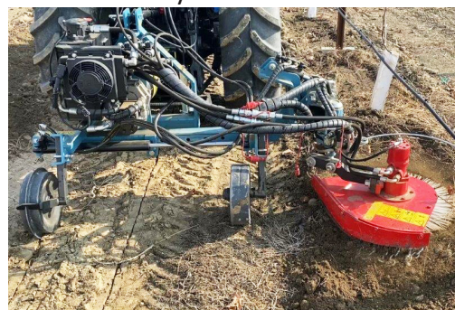
Rotary Hoe at work
